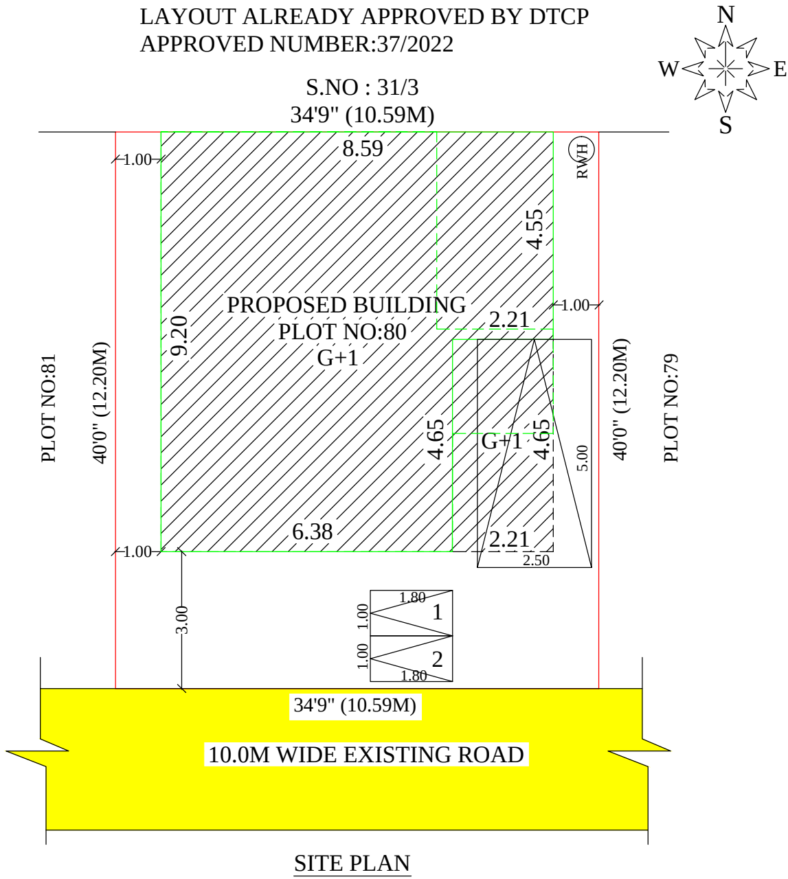
SITE PLAN
