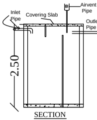
SECTION OF RAIN WATER COLLECTION PITS
