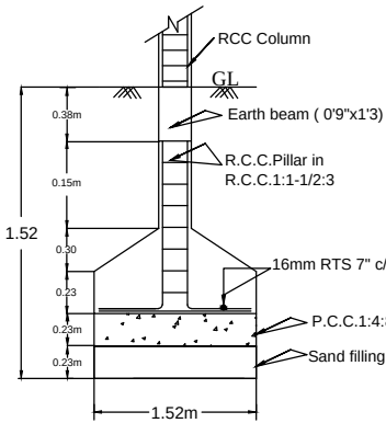
FOUNDATION DETAILS
