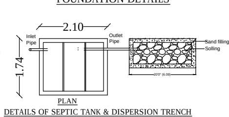
DETAILS OF SEPTIC TANK & DISPERSION TRENCH
