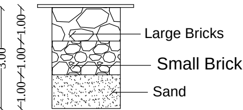
SECTION OF RAIN WATER COLLECTION PITS
