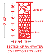
SECTION OF RAIN WATER COLLECTION PITS (NTS)
