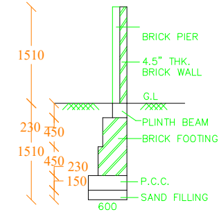
COMPOUND WALL DETAIL SCALE : 1" = 2'-0"
