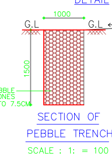
SECTION OF PEBBLE TRENCH SCALE : 1" = 100'
