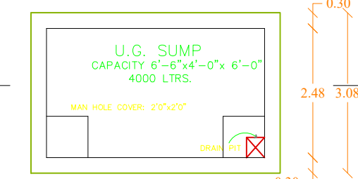
U.G. SUMP CAPACITY 6'-6"x4'-0"x 6'-0" 4000 LTRS. SCALE 1"=4'0"
