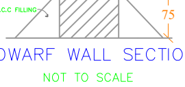
DWARF WALL SECTION NOT TO SCALE
