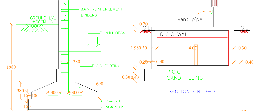
TYPICAL SECTION OF R.C.C COLUMN FOUNDATION SCALE : 1" = 2'-0"
