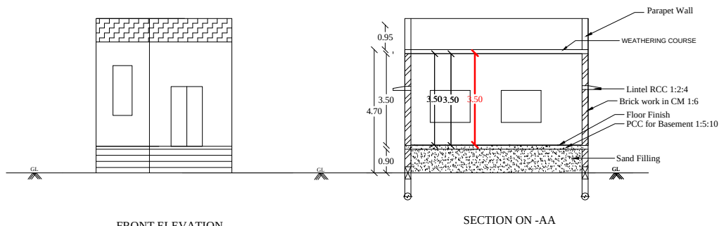
FRONT ELEVATION
