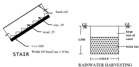
RAINWATER HARVESTING
