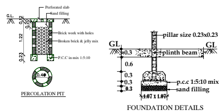
FOUNDATION DETAILS
