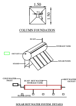
SOLAR HOT WATER SYSTEM DETAILS
