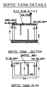
SEPTIC TANK PLAN
