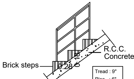
STAIRCASE DETAILS
