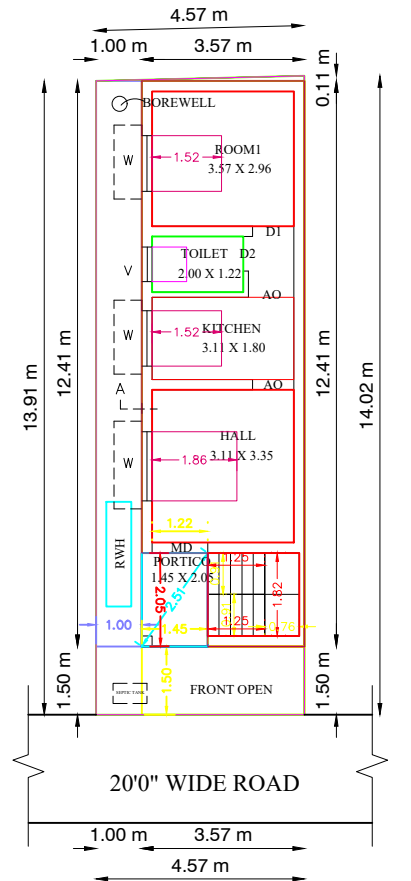
PRO. GROUND FLOOR PLAN
