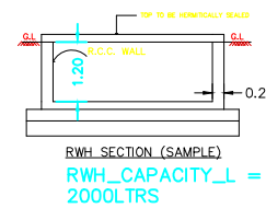
RW SECTION (SAMPLE) RW_CAPACITY_L = 2000LTRS
