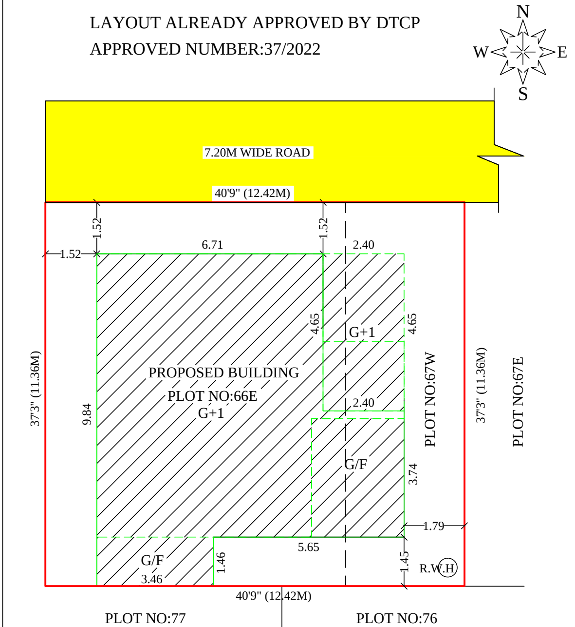
SITE PLAN
