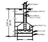
FOUNDATION DETAILS
