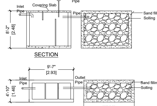
DETAILS OF SEPTIC TANK & DISPERSION TRENCH
