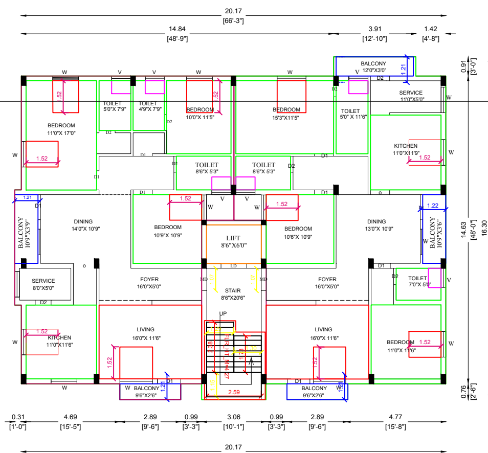
TYPICAL FLOOR PLAN ( FIRST, SECOND, THIRD )
