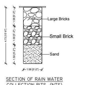
SECTION OF RAIN WATER COLLECTION (R.T.S. - INTS)
