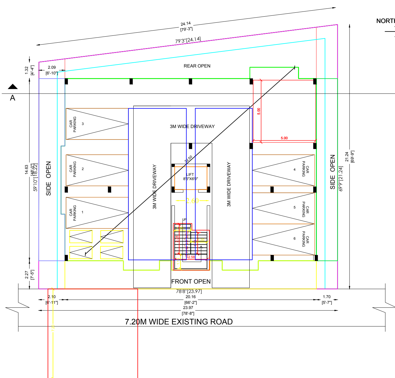
SITE CUM STILT FLOOR PLAN
