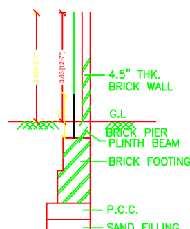
COMPOUND WALL
