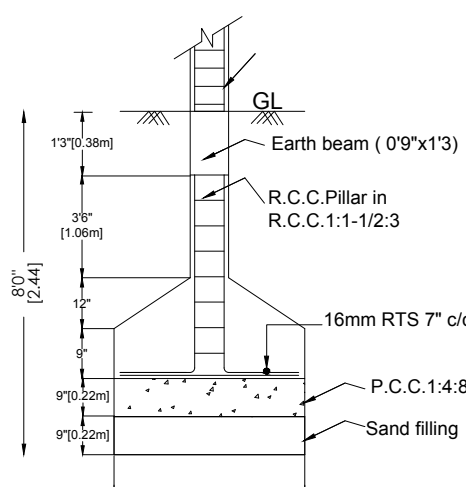
FOUNDATION DETAILS
