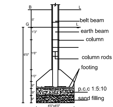
FOUNDATION DETAILS
