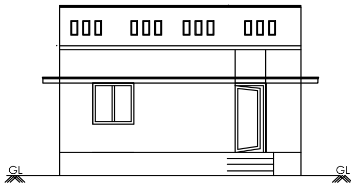
FRONT ELEVATION
