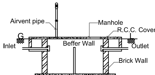
SEPTIC TANK PLAN DETAILS
