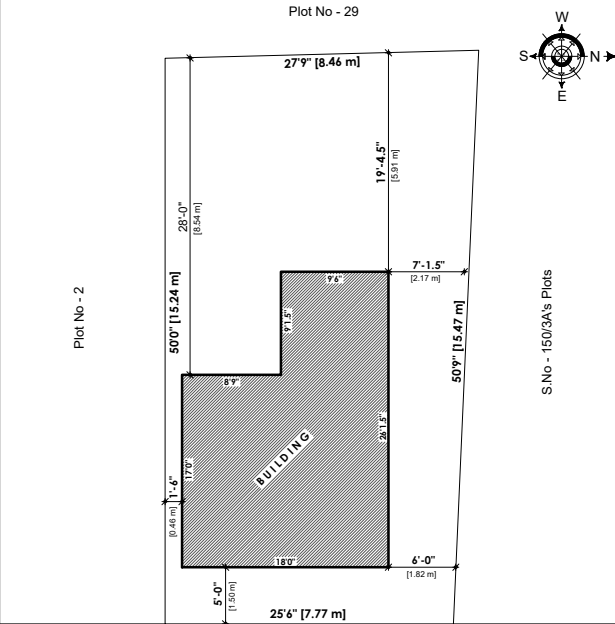
SITE PLAN
