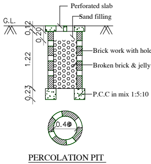
PERCOLATION PIT
