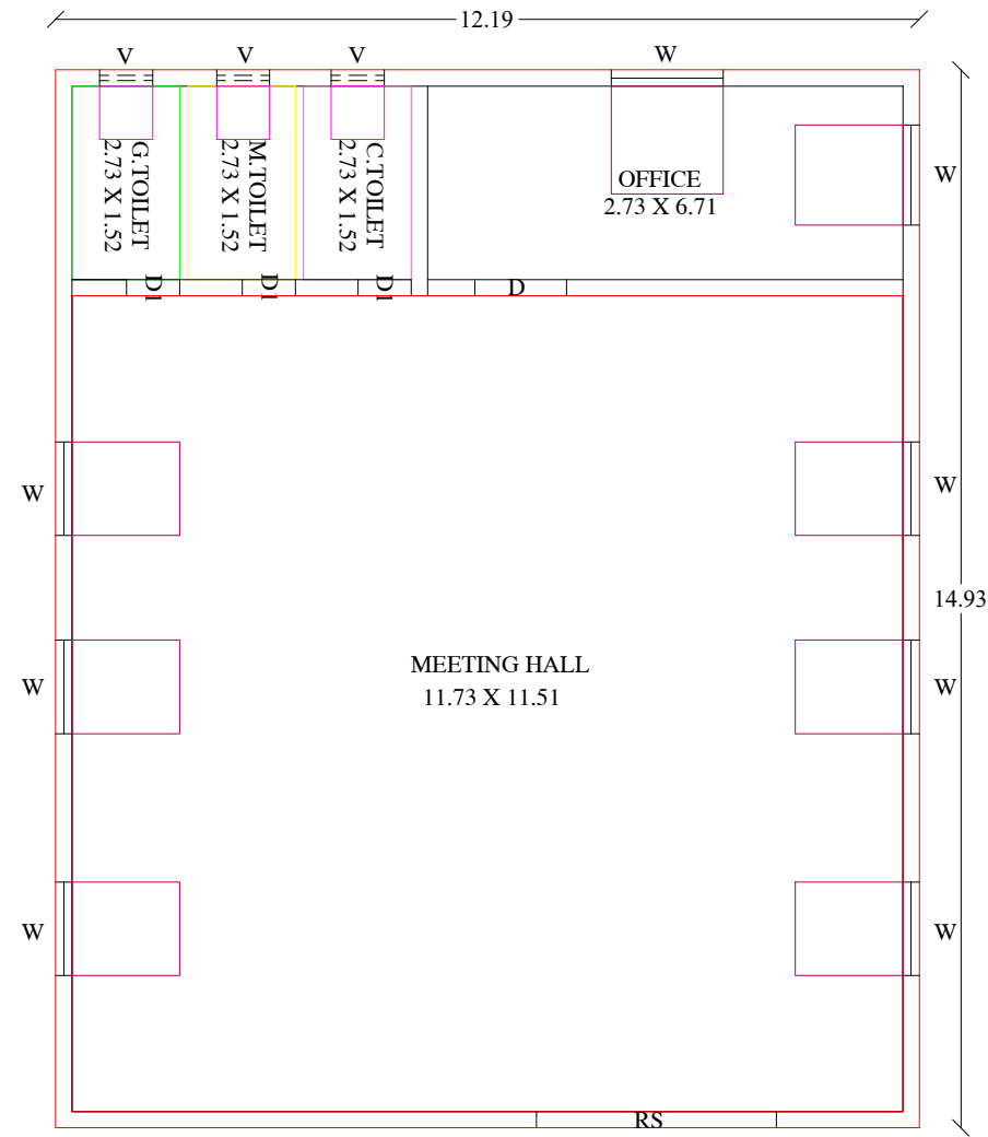
GROUND FLOOR PLAN (EAST FACING)
