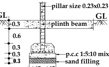
FOUNDATION DETAILS
