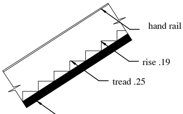
STAIR
