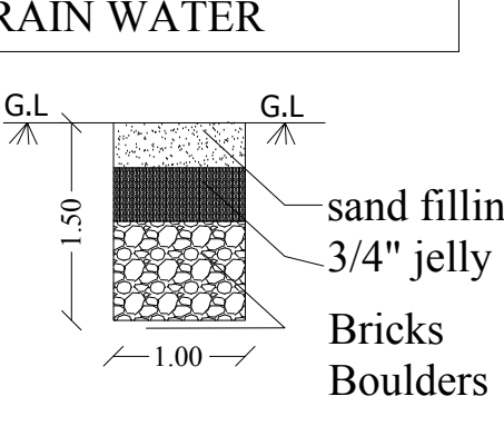
TRIAL PIT
