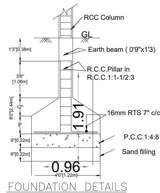
FOUNDATION DETAILS
