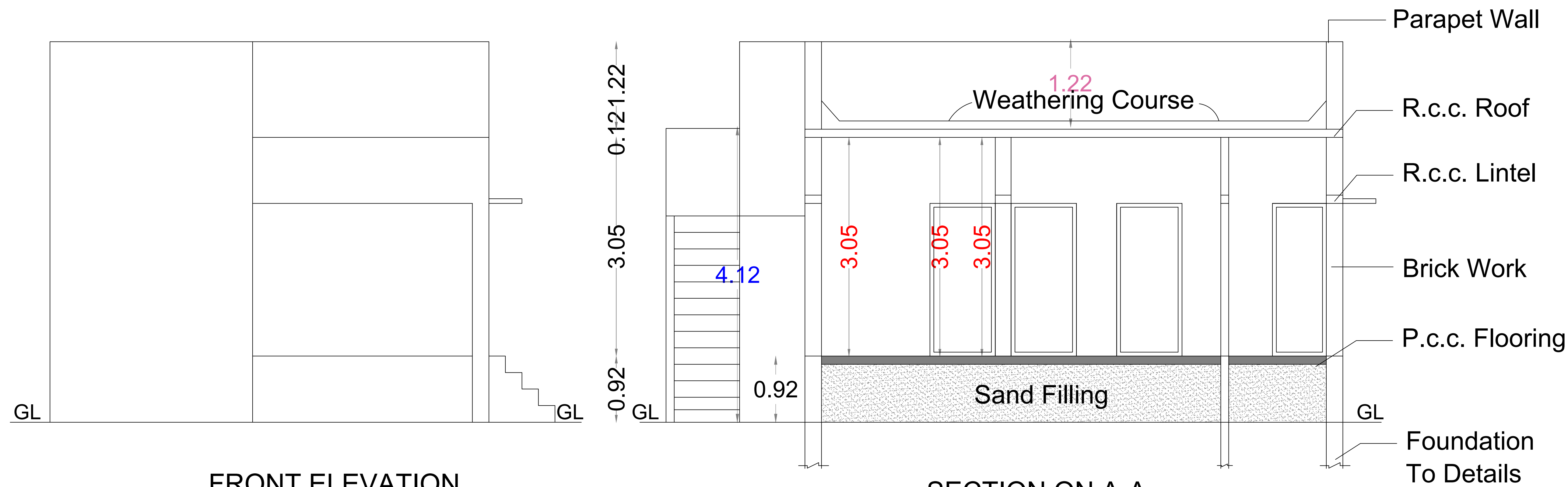
SECTION ON A-A
