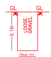
TRIAL PIT
