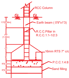
FOUNDATION DETAILS
