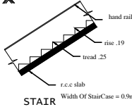
STAIR
