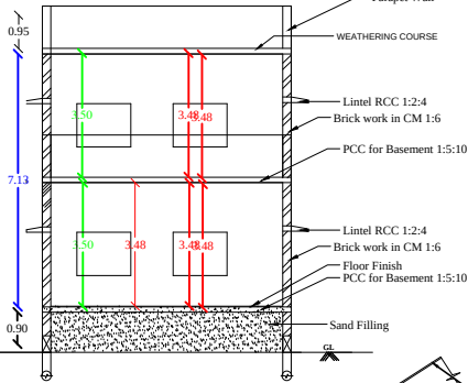
SECTION ON-AA
