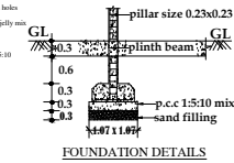
FOUNDATION DETAILS
