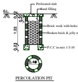
PERCOLATION PIT
