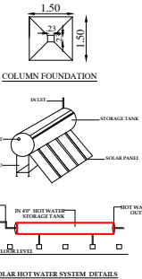
SOLAR HOT WATER SYSTEM DETAILS
