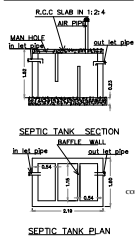
SEPTIC TANK PLAN
