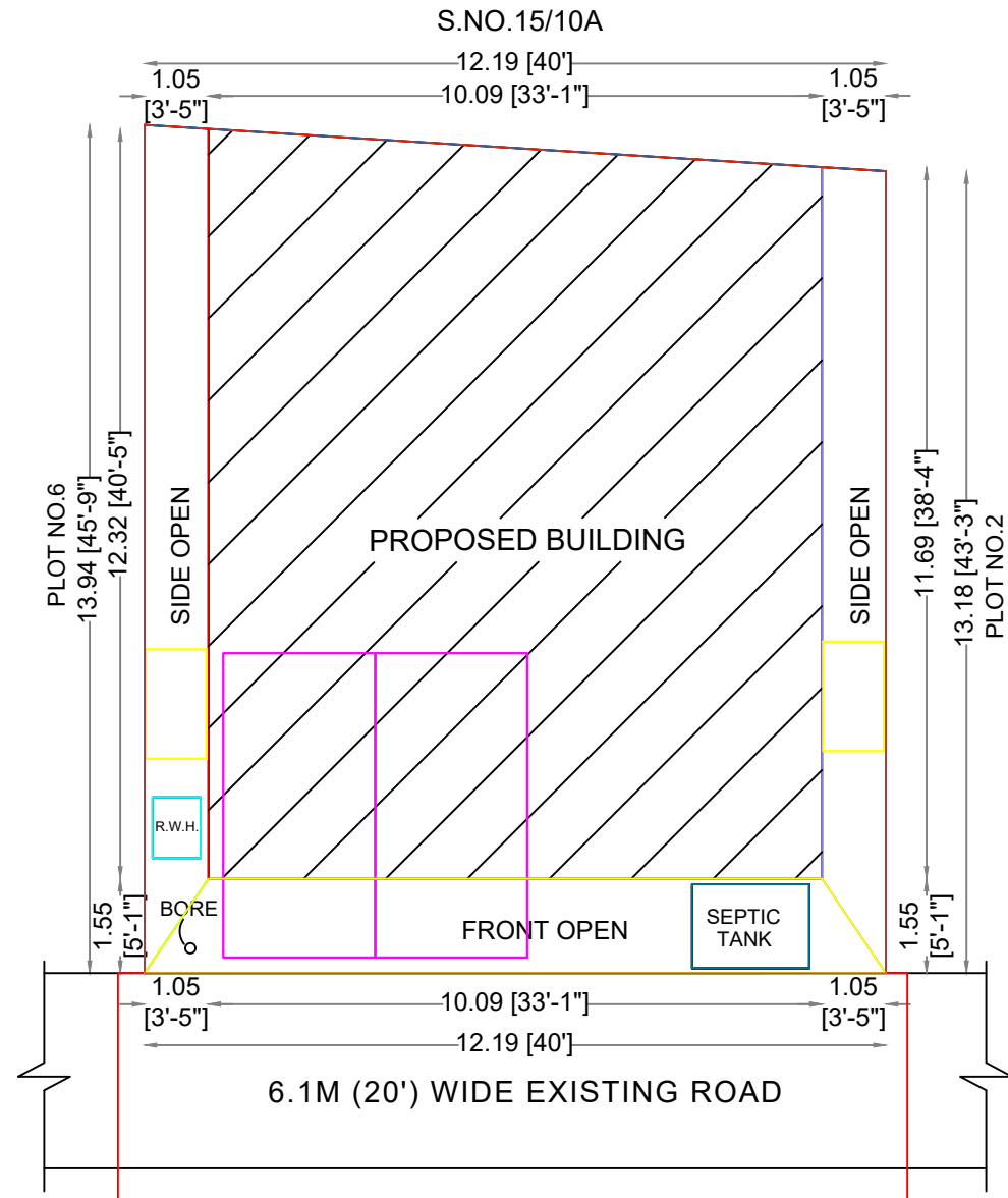
SITE PLAN
