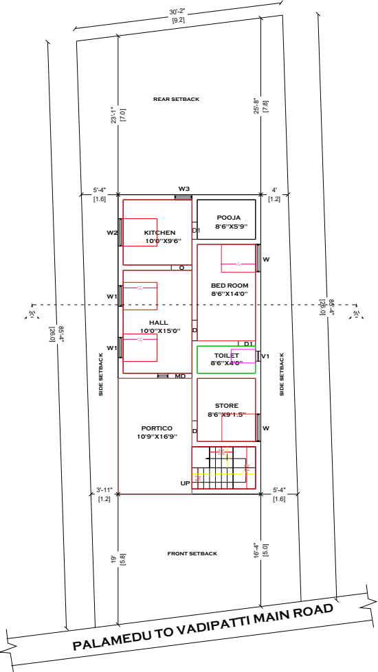
EXI. GROUND FLOOR PLAN
