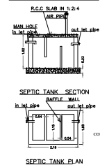
SEPTIC TANK PLAN
