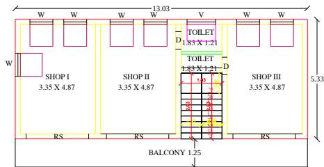
GROUND FLOOR PLAN (EAST FACING)
