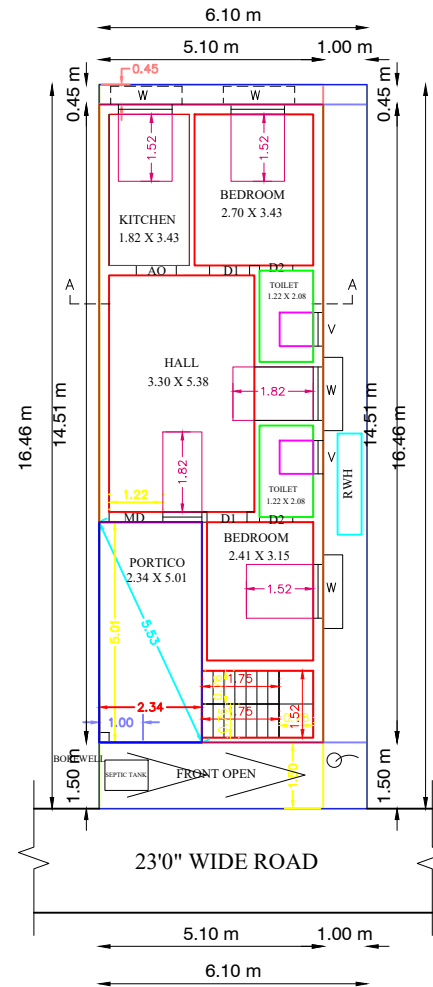
PRO.GROUND FLOOR PLAN
