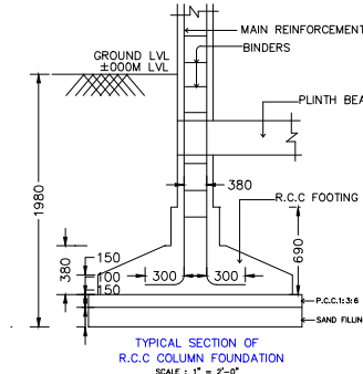
TYPICAL SECTION OF R.C.C COLUMN FOUNDATION SCALE : 1" = 2'-0"
