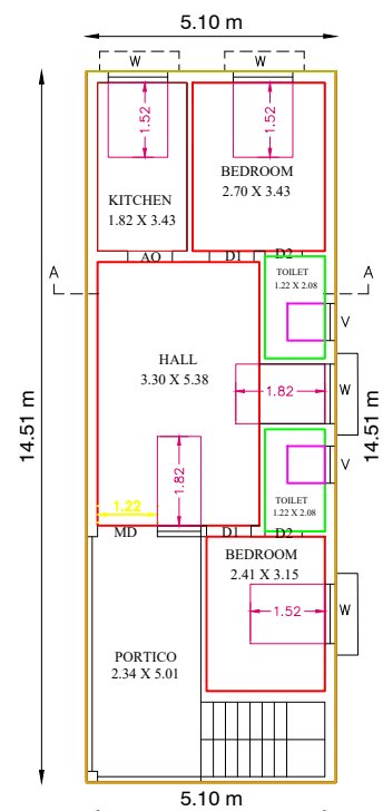
PRO.FIRST FLOOR PLAN
