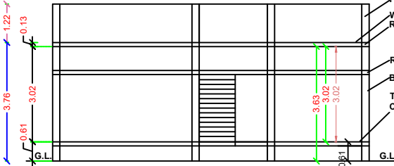
SECTION ON B-B
