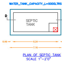
PLAN OF SEPTIC TANK SCALE 1"=2'0"
