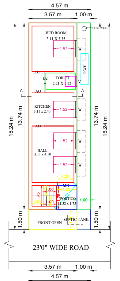
PRO.GROUND FLOOR PLAN
