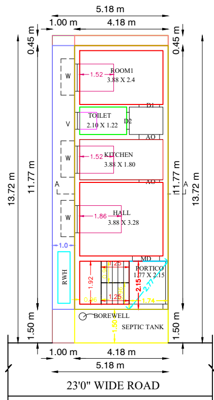
PRO. GROUND FLOOR PLAN
