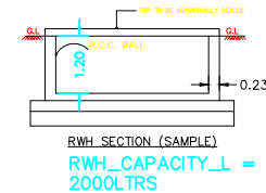
RWHT SECTION (SAMPLE) RWHT_CAPACITY_L = 2000LTRS
