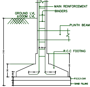
TYPICAL SECTION OF R.C.C. COLUMN FOUNDATION
