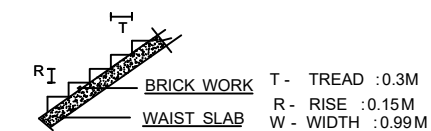
STAIRCASE DETAILS
