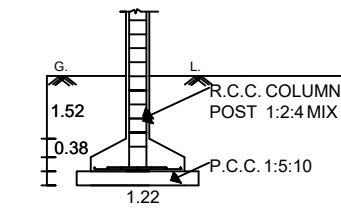
FOUNDATION DETAILS
