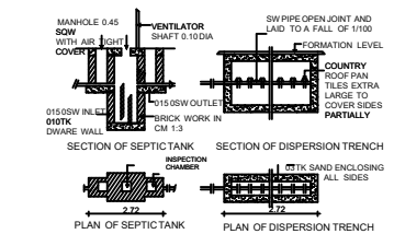
DRAWING FOR SEPTIC TANK WITH DISPERSION TRENCH
