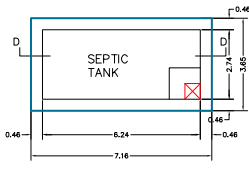
PLAN OF SEPTIC TANK SCALE 1"=2'0"
