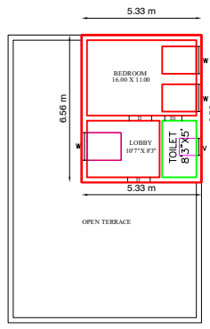
PRO.SECOND FLOOR PLAN
