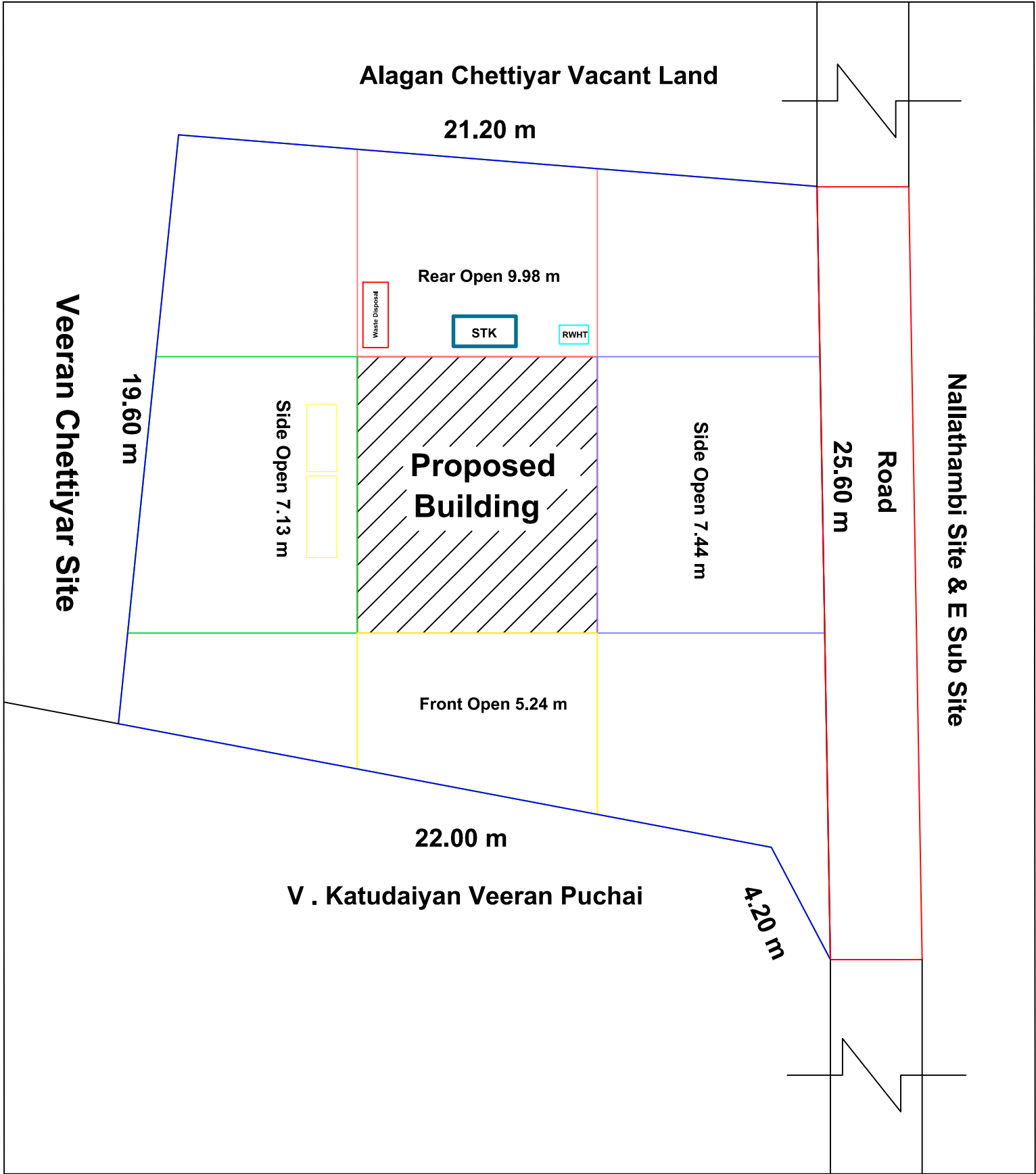
Site Plan
