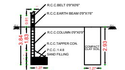
FOUNDATION DETAILS-END COLUMN
