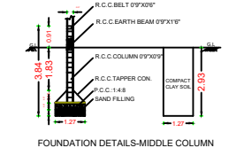
FOUNDATION DETAILS-MIDDLE COLUMN
