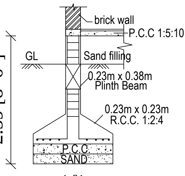
FOUNDATION DETAILS
