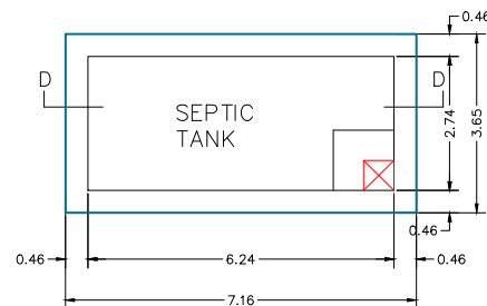
PLAN OF SEPTIC TANK SCALE 1"=2'0"
