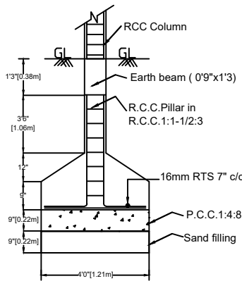
FOUNDATION DETAILS
