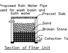
Section of Filter Unit
