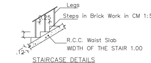
STAIRCASE DETAILS
