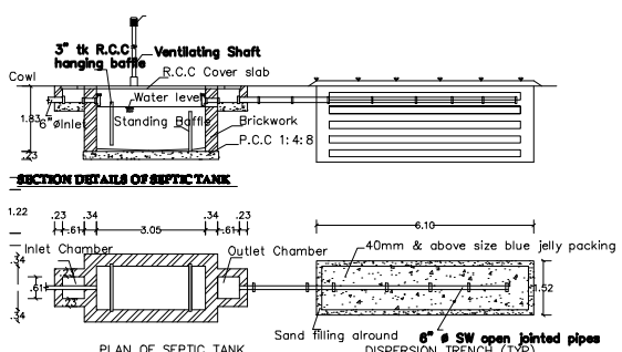
DETAILS OF SEPTIC TANK & DISPERSION TRENCH
