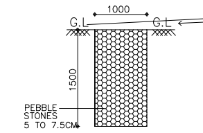
SECTION OF PEBBLE TRENCH SCALE : 1: = 100
