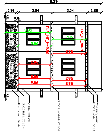
SECTION ON R.R.
