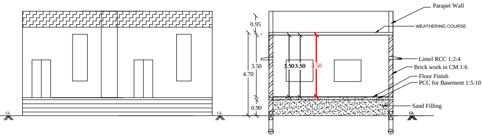
SECTION ON-AA
