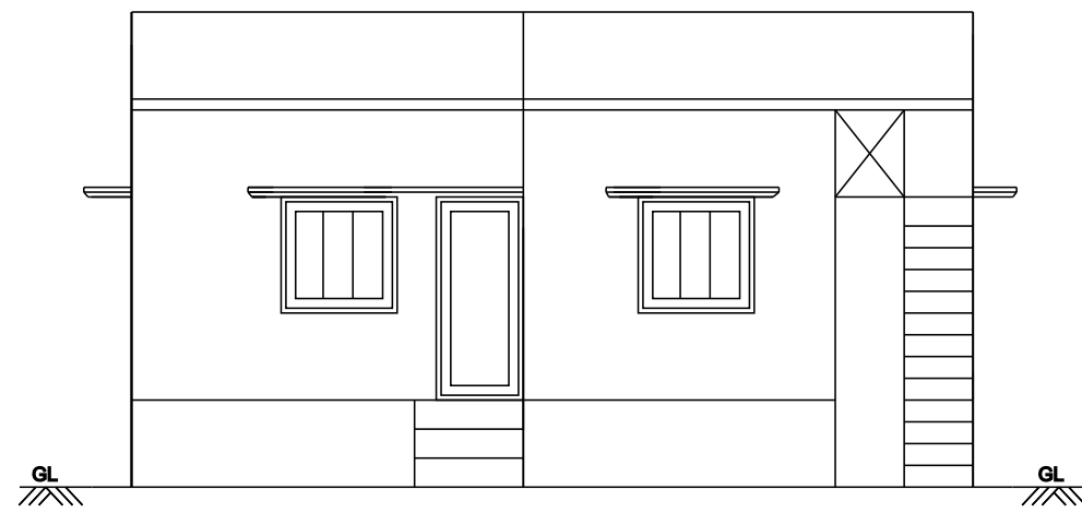
FRONT ELEVATION
