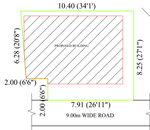
SITE PLAN
