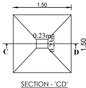
SECTION - "CD"
