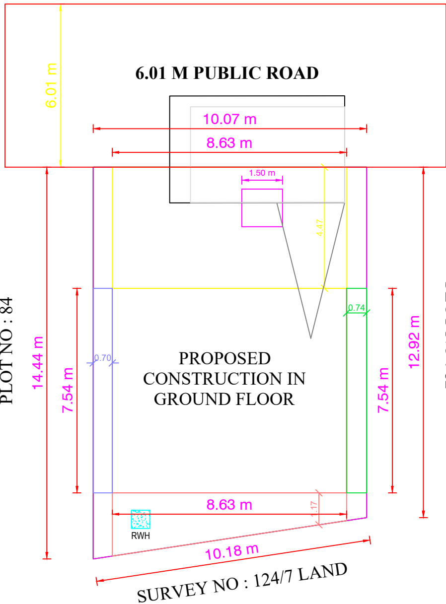
SITE PLAN
