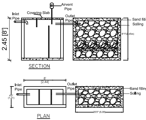
DETAILS OF SEPTIC TANK & DISPERSION TRENCH
