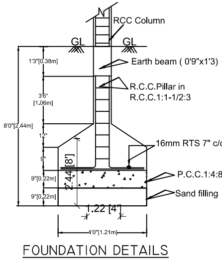
FOUNDATION DETAILS
