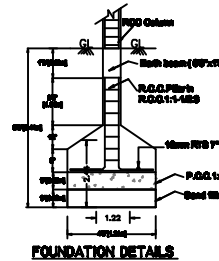
FOUNDATION DETAILS
