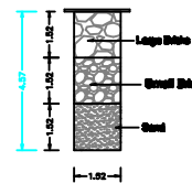
SECTION OF RAIN WATER COLLECTION PIPE (RWT) RWT_CAPACITY_L = 2000.00
