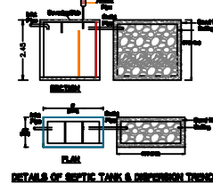
DETAILS OF SEPTIC TANK & DISPERSION TRENCH
