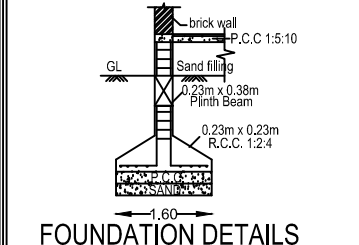
FOUNDATION DETAILS
