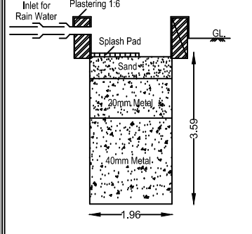
RAIN WATER PERCOLATION PIT
