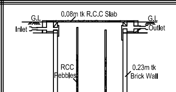
SECTION OF SEPTIC TANK
