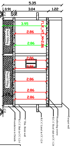
SECTION ON RK
