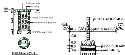
FOUNDATION DETAILS
