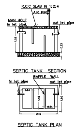
SEPTIC TANK PLAN
