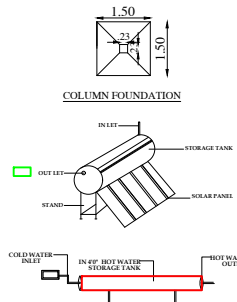
SOLAR HOT WATER SYSTEM DETAILS
