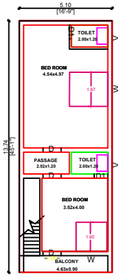
PRO.FIRST FLOOR PLAN
