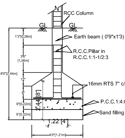
FOUNDATION DETAILS
