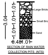
SECTION OF RAIN WATER COLLECTION PITS (INTS)
