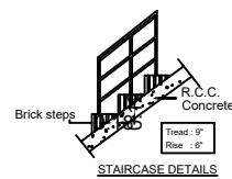
STAIRCASE DETAILS
