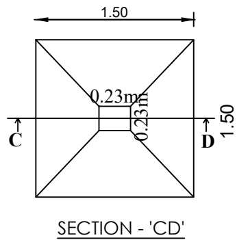
SECTION - 'CD'
